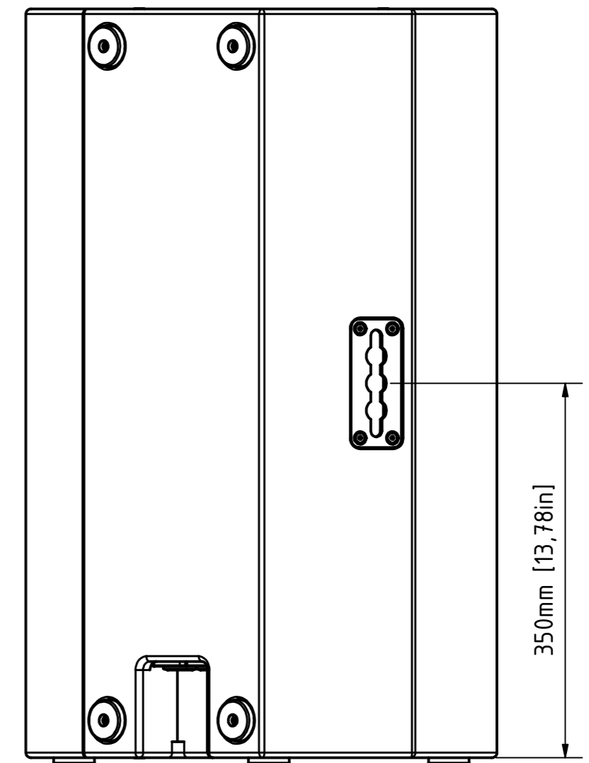
rear view
