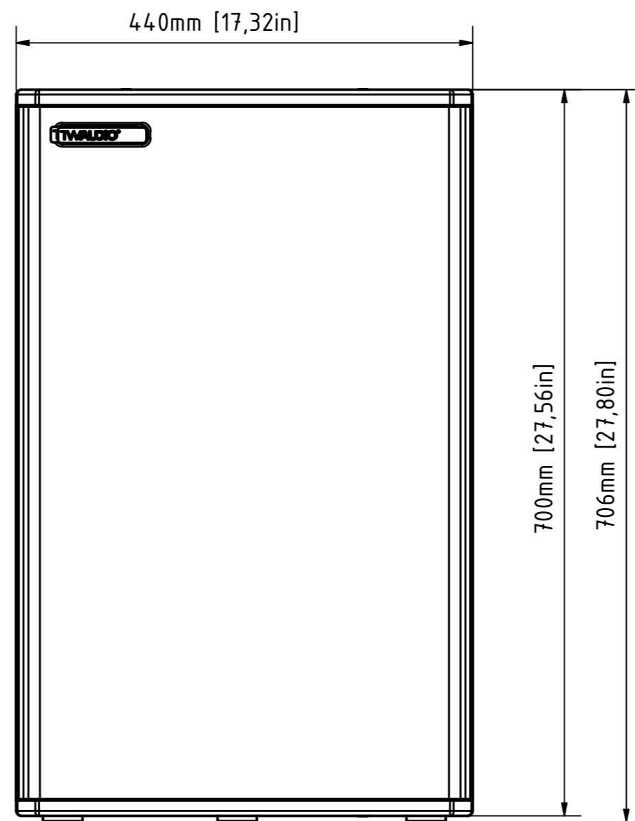
front view
