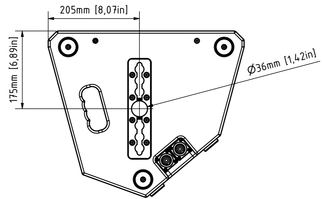
bottom view
