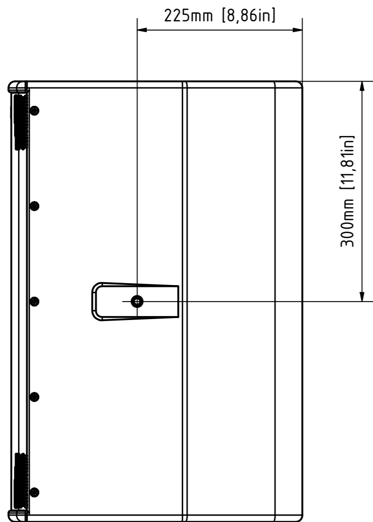
right view
