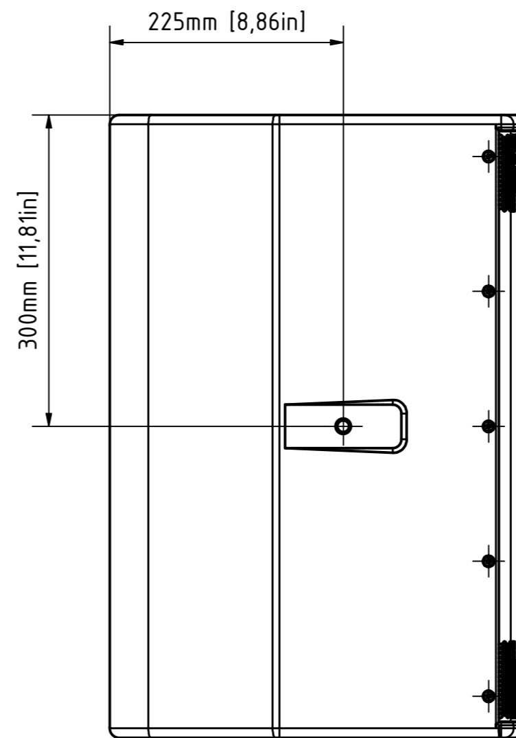
left view
