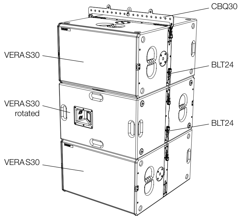
Figure 4.4 - System setup CBQ30 with VERAS30 loudspeaker - cardioid mode
