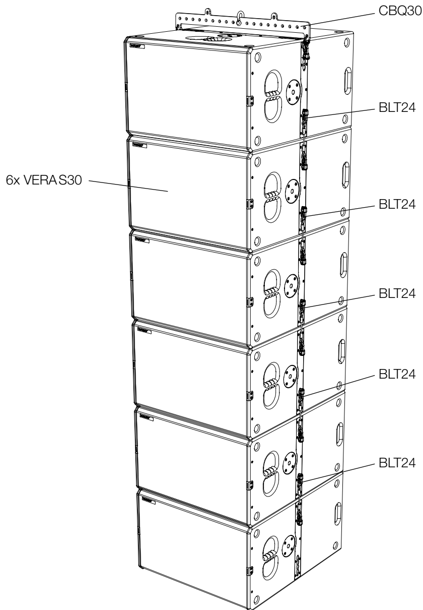
Figure 4.3 - System setup CBQ30 with VERAS30 loudspeaker
