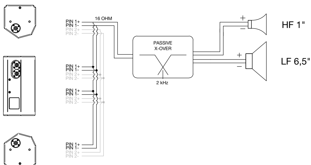
Figure 3.2 - Connection diagram
