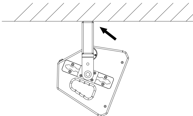
Figure 4.5 - Assembly QBM10 with M10 to ceiling
