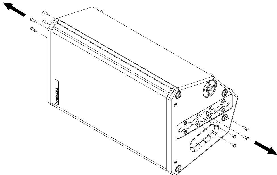
Figure 4.4.1 - Removing the countersunk screws on the M10 loudspeaker
