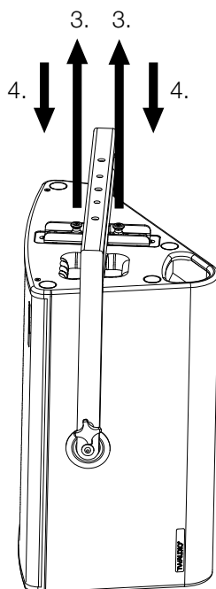
Figure 4.3 - Assembly SBC15 to C15 loudspeaker
