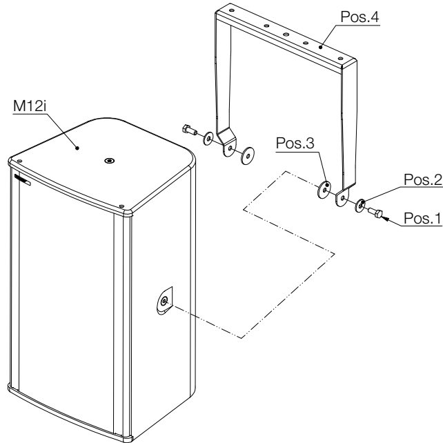
Figure 4.5 - Assembly SBM12i to M12i loudspeaker
