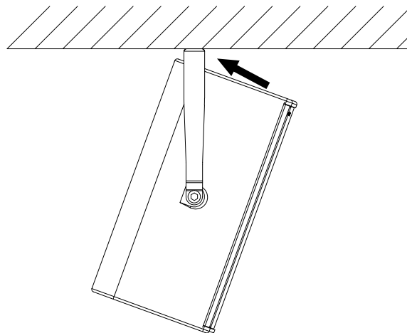
Figure 4.6 - Assembly SBM12i with M12i to ceiling
