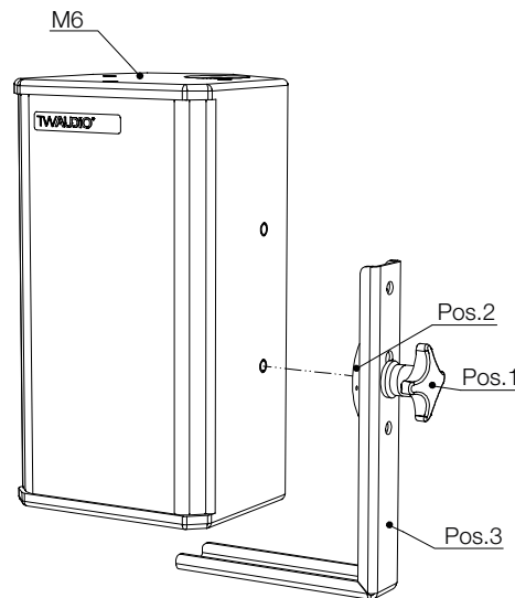
Figure 4.5 - Assembly SBM6 to M6 loudspeaker
