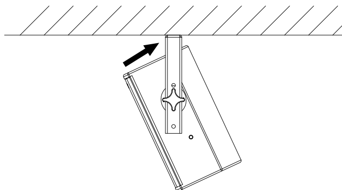
Figure 4.6 - Assembly SBM6 with M6 to ceiling
