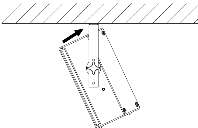
Figure 4.6 - Assembly SBM8 with M8 to ceiling
