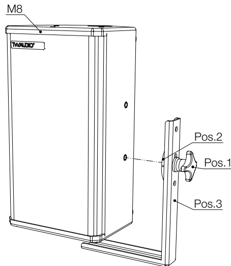
Figure 4.5 - Assembly SBM8 to M8 loudspeaker
